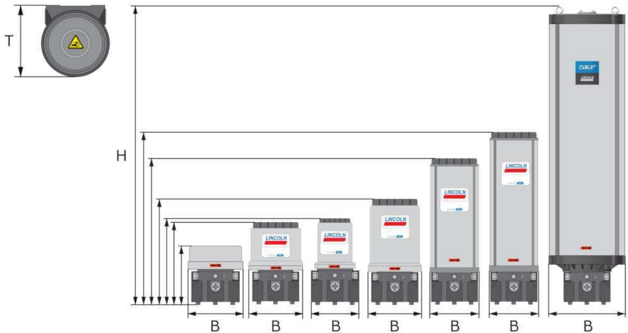
Minimum mounting dimensions
