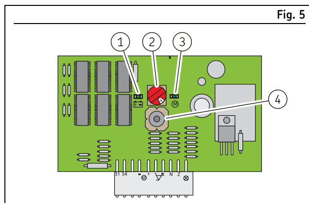
Control circuit board H
