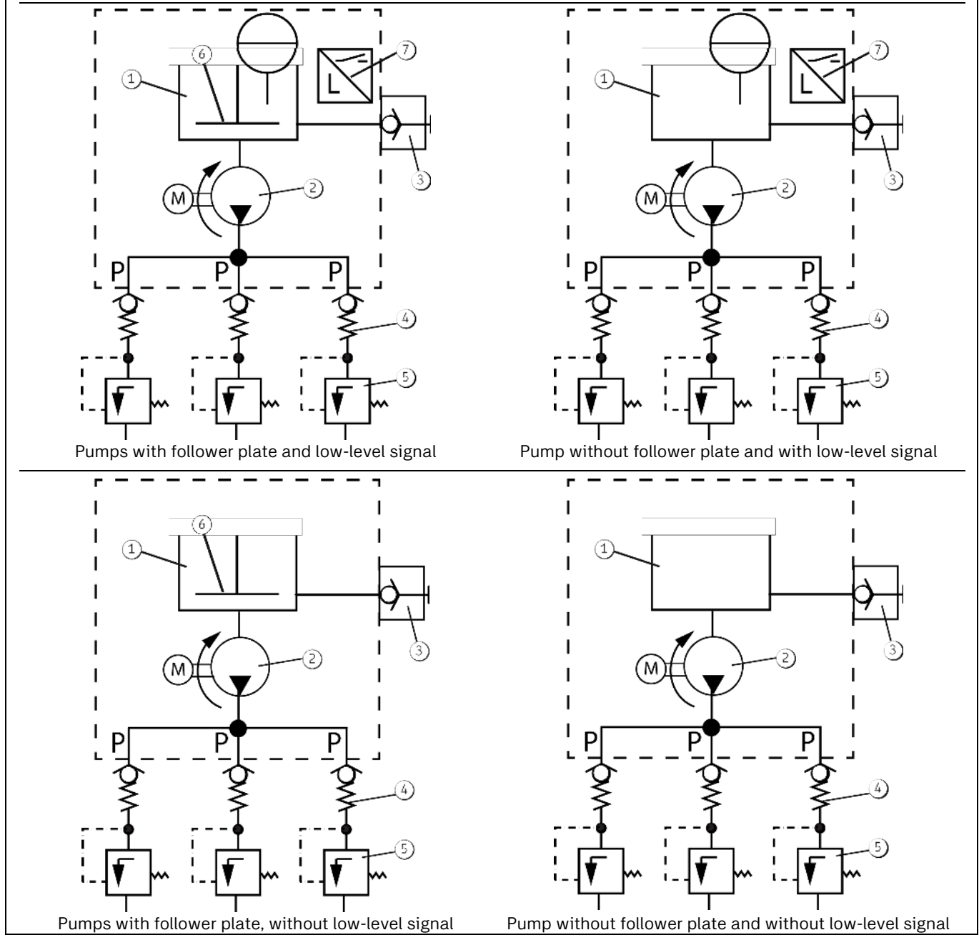
Hydraulic connection diagrams
