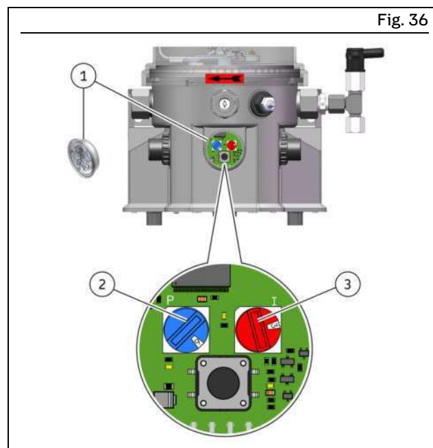
P203 with control circuit board V10-V23
