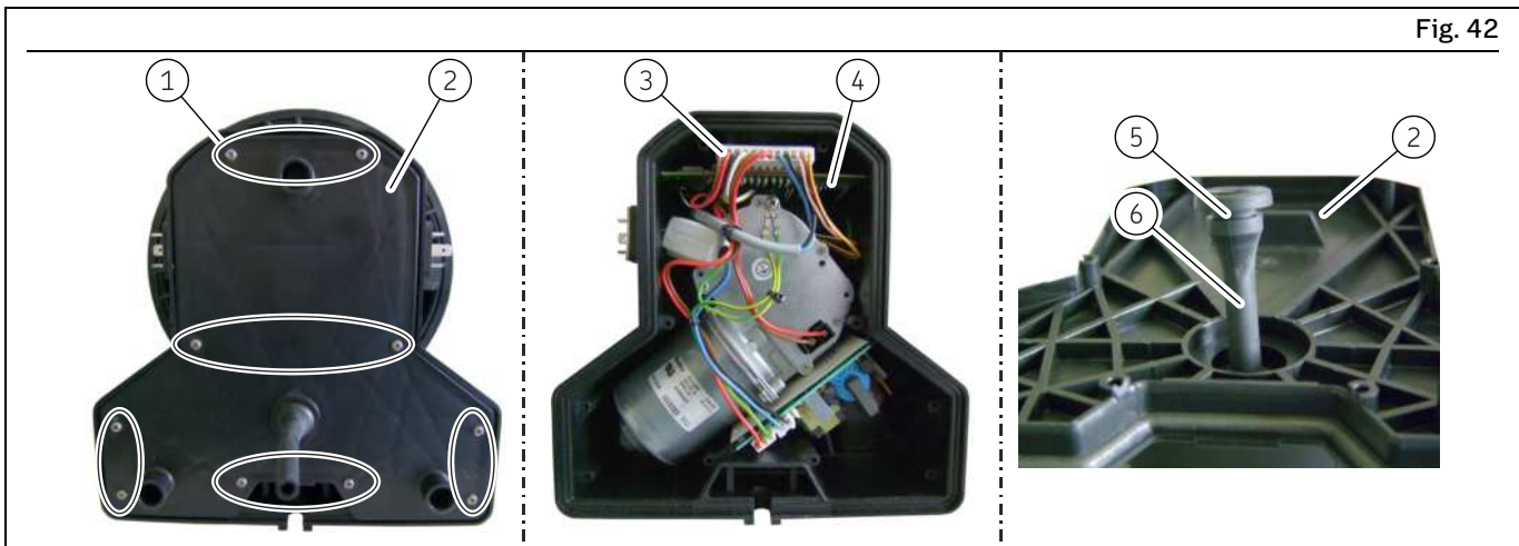
Replacing the control circuit board
