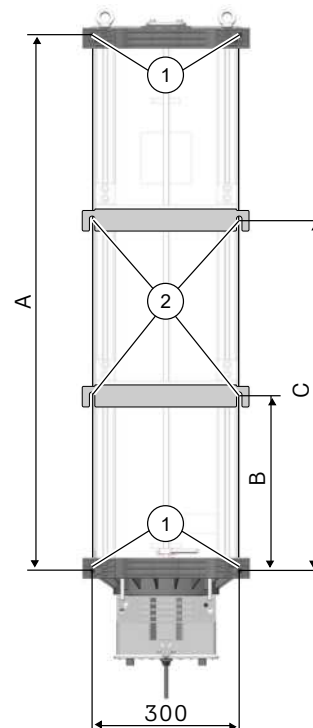
Assembly holes P203 with Xx_G- / XBxG reservoir
